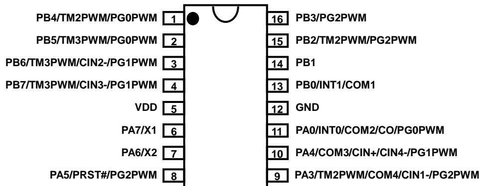
PMS154C-S16: SOP16 (150mil)
