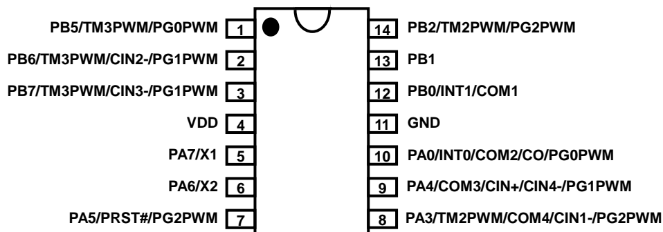
PMS154C-S14: SOP14 (150mil)
